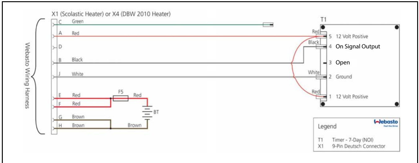
Wiring diagram - NOI (No Operator Interface) Timer
