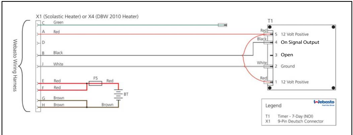
Wiring diagram - NOI (No Operator Interface) Timer
